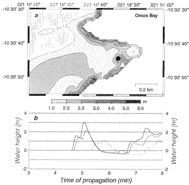
Figure 3. (a) Maximal water heights computed in Omoa Bay after an 8-min propagation are shown with 1-m contours. The dashed white line corresponds to the shoreline at rest. The white triangle displays the location of the school where waves at least 3-m high were reported. The numerical gage used during the computation is shown as the black disk. (b) Water heights obtained at this gage for the 0.0024-km 3 event simulation (solid line), the 0.0012-km 3 event simulation (dashed line), and the shifted 0.0024-km 3 event (dotted line) are plotted as a function of the propagation time.
