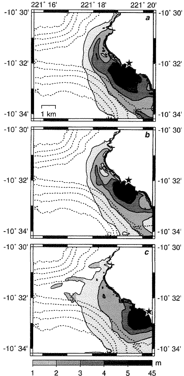
Figure 4. Maximal water heights are shown after an 8-min modeling time, for the 0.0024-km 3 event (a), the 0.0012-km 3 event (b), and the 0.0024-km 3 shifted event (c) (in this case, the longitudinal extent of the computational domain has been increased). Note that the gray scale is not linear to deal with high values reached around the area of failure. Dashed lines are the bathymetric values contoured at 200 m intervals.
